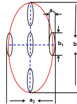
Figure 2: Schematic illustration of a 2D cross section through the 3D ellipsoidal crack distribution in the T-matrix model. The aspect ratio of the individual cracks is a_1/b_1 , and the aspect ratio of the crack distribution is a_2/b_2 (After Hu and McMechan, 2009).
