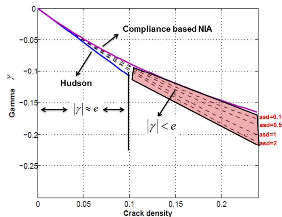
Figure 9: Comparisons of predictions of Thomsen's anisotropic parameter Gamma as a function of crack density. Black dashed lines indicate T-matrix prediction with different aspect ratio of spatial distribution marked.
