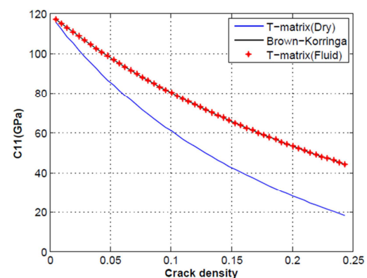
Figure 6: Illustration of T-matrix to Biot-consistency. The effective elastic stiffness C_{11} is displayed as a function of crack density.
